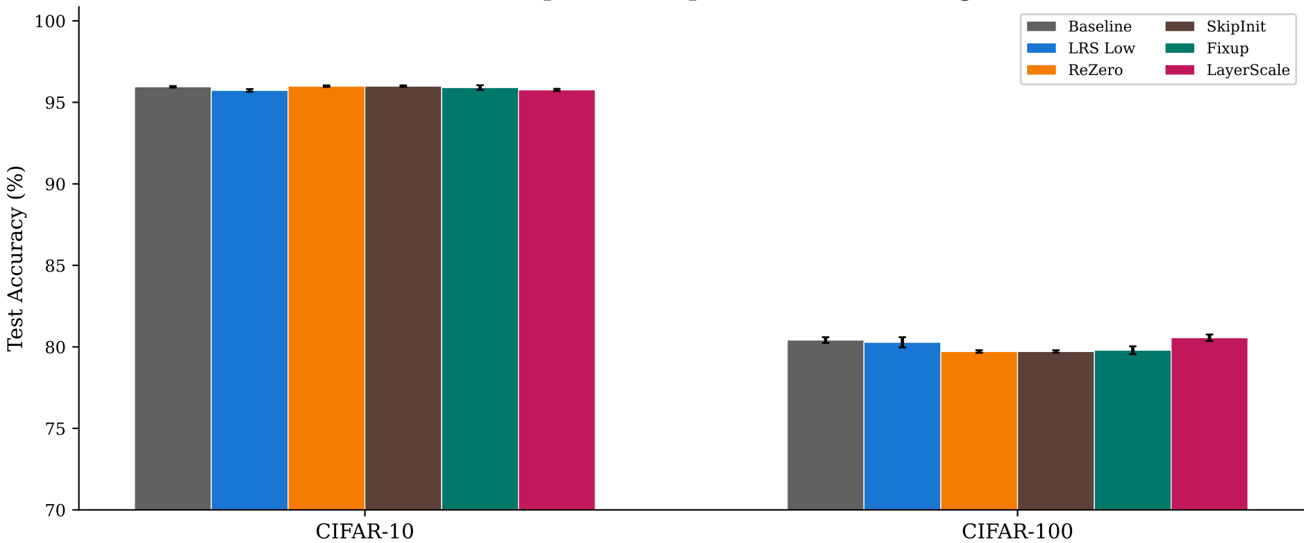
Method Comparison (Depth 152, 3-seed Average)
