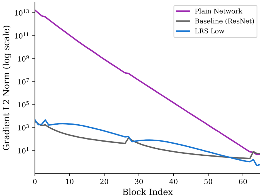
(a) Gradient Flow Comparison
