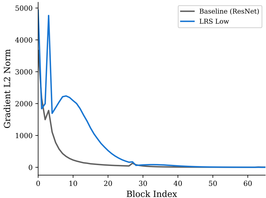
(b) ResNet vs LRS (Linear Scale)
