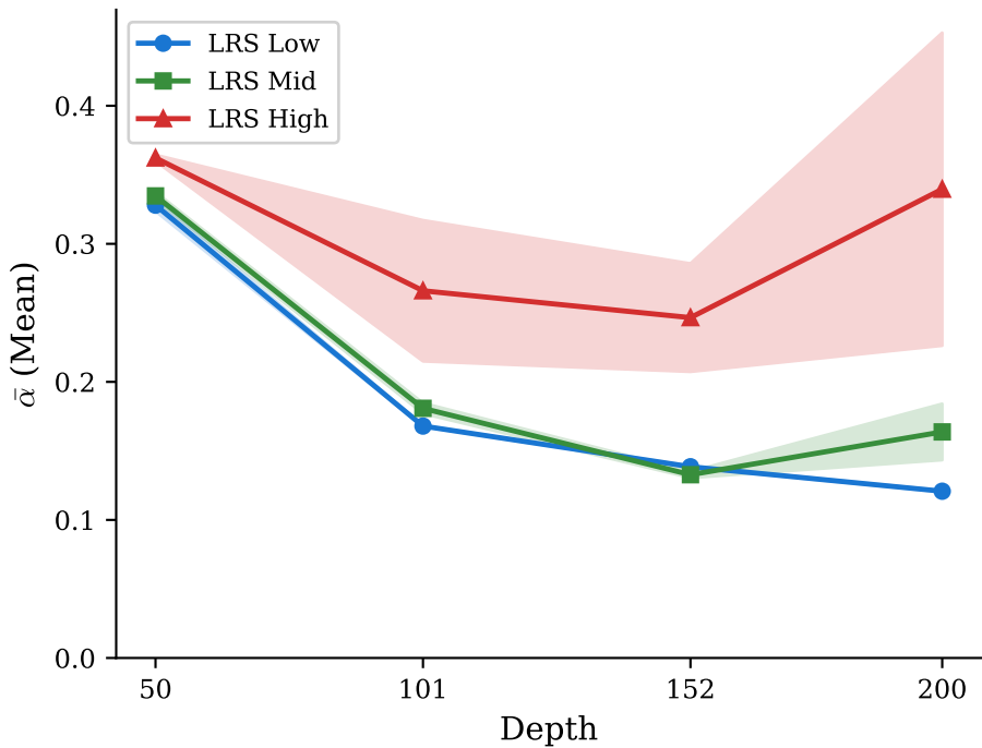
CIFAR-10
