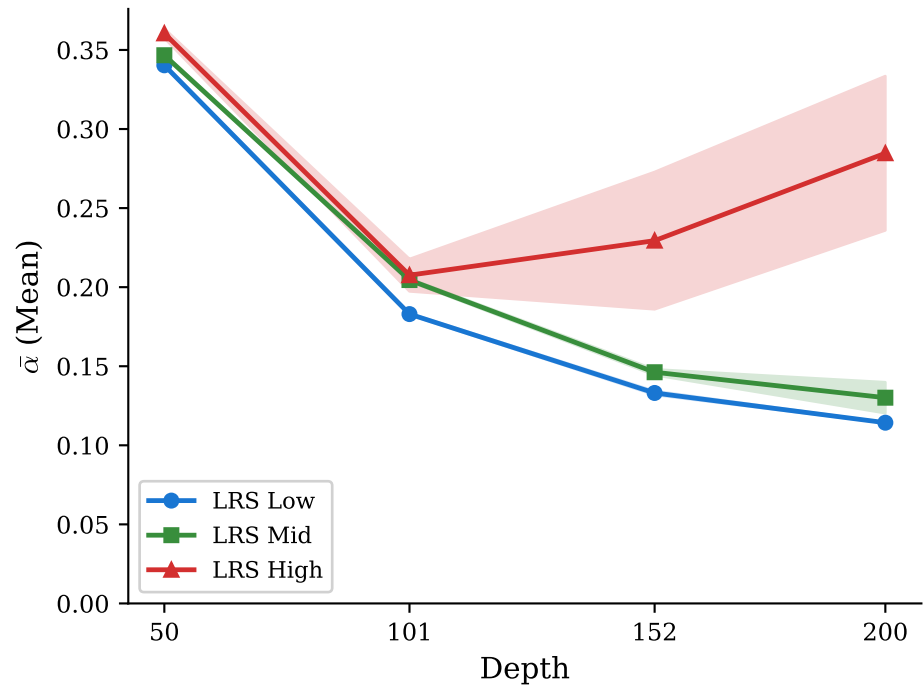
CIFAR-100
