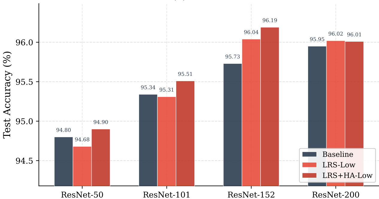
(a) CIFAR-10
