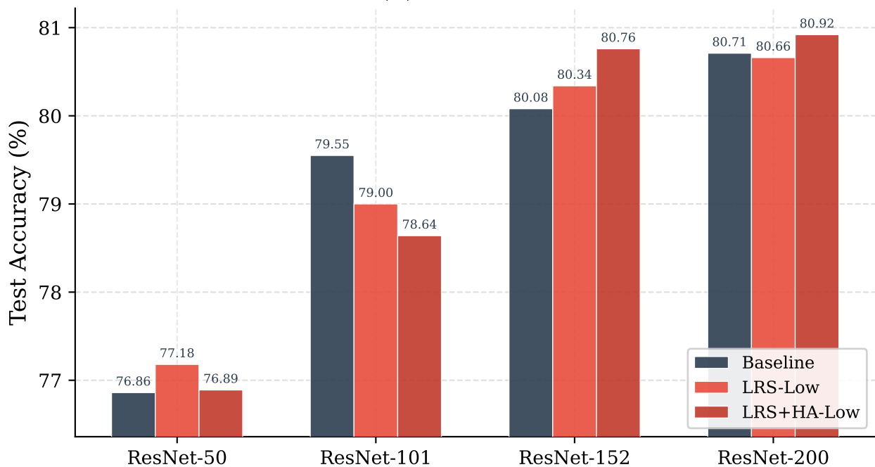
(b) CIFAR-100
