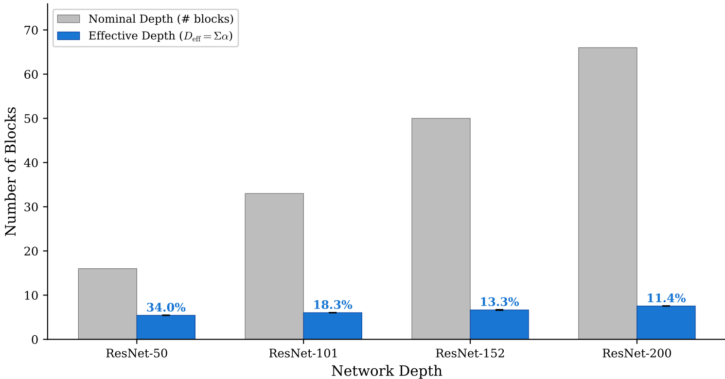
Effective Depth vs Nominal Depth (LRS Low, CIFAR-100)
