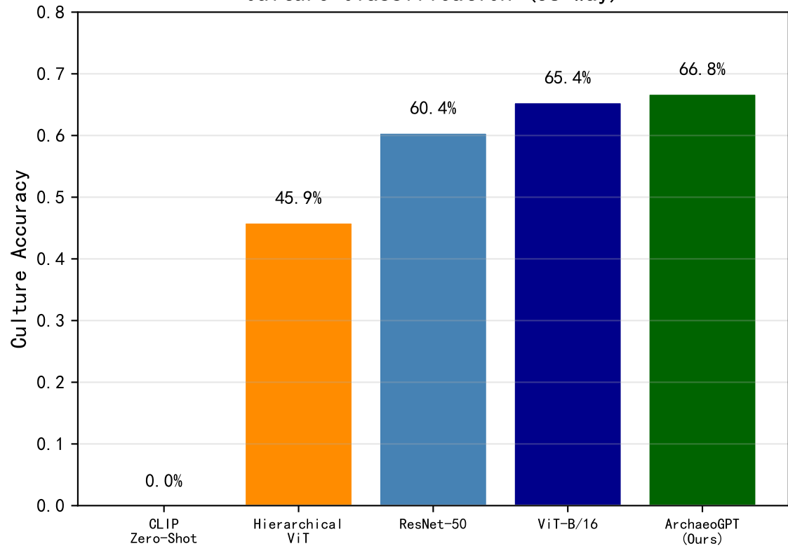
Culture Classification (58-way)
