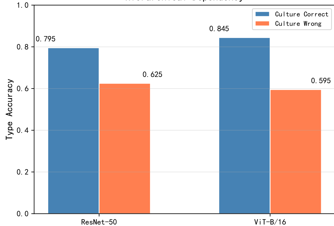
Hierarchical Dependency
