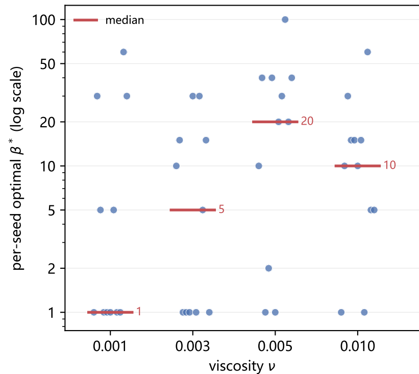
(b) Per-seed optimal \beta^* : dispersed and non-monotone
