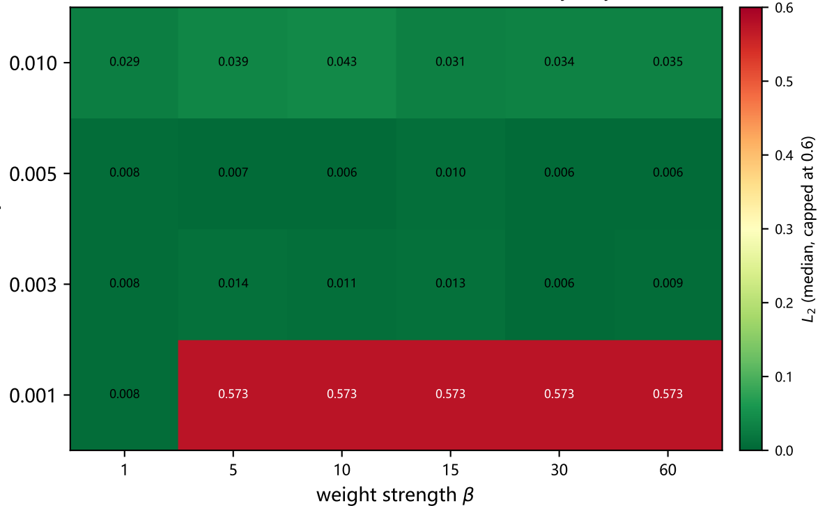
(a) Cell-median terminal L_2 (central tendency only)
