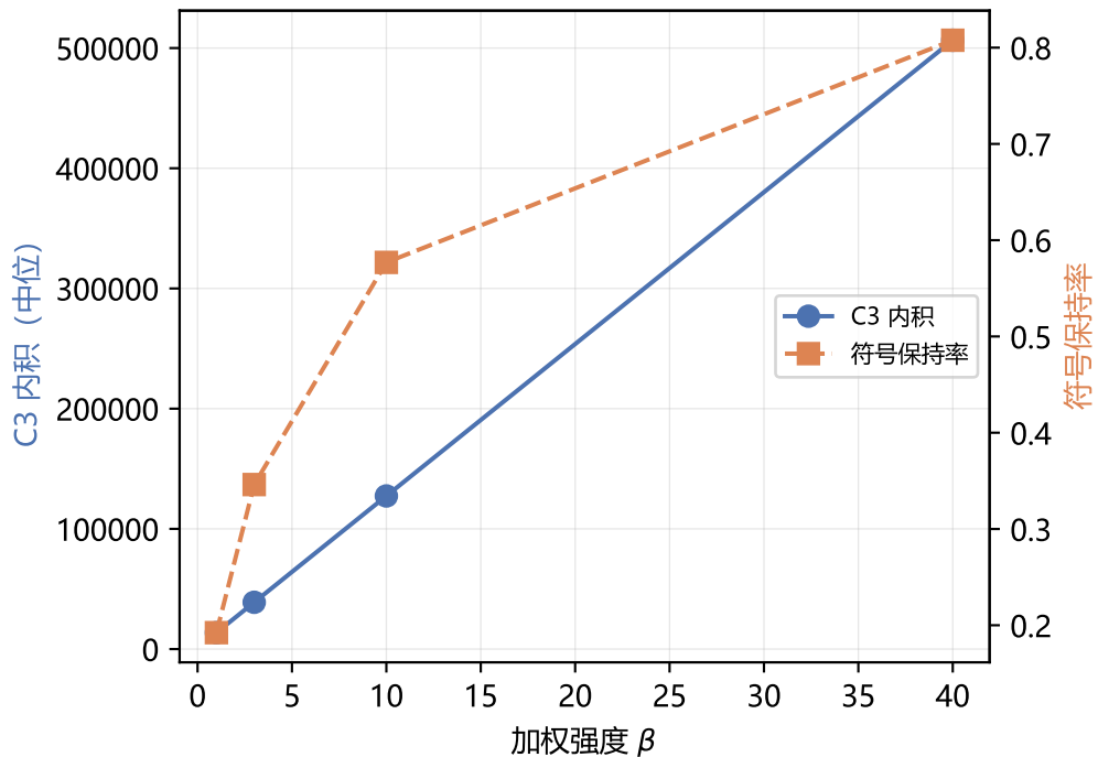
(b) G3: C3 机制验证
