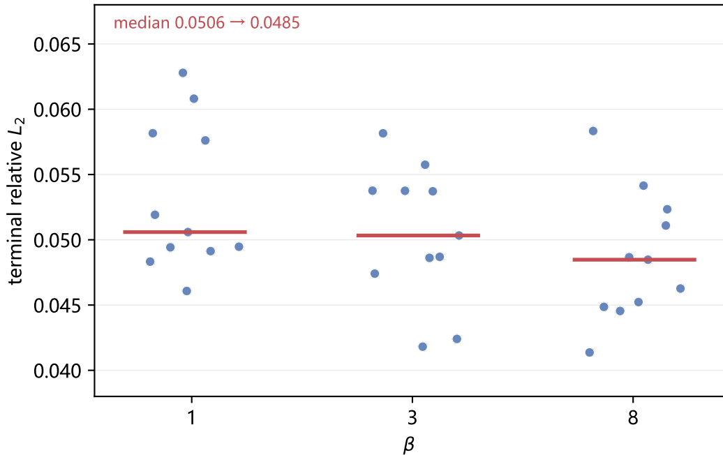
C4/C5 2-D linear advection–diffusion: all 33 runs in good basins
