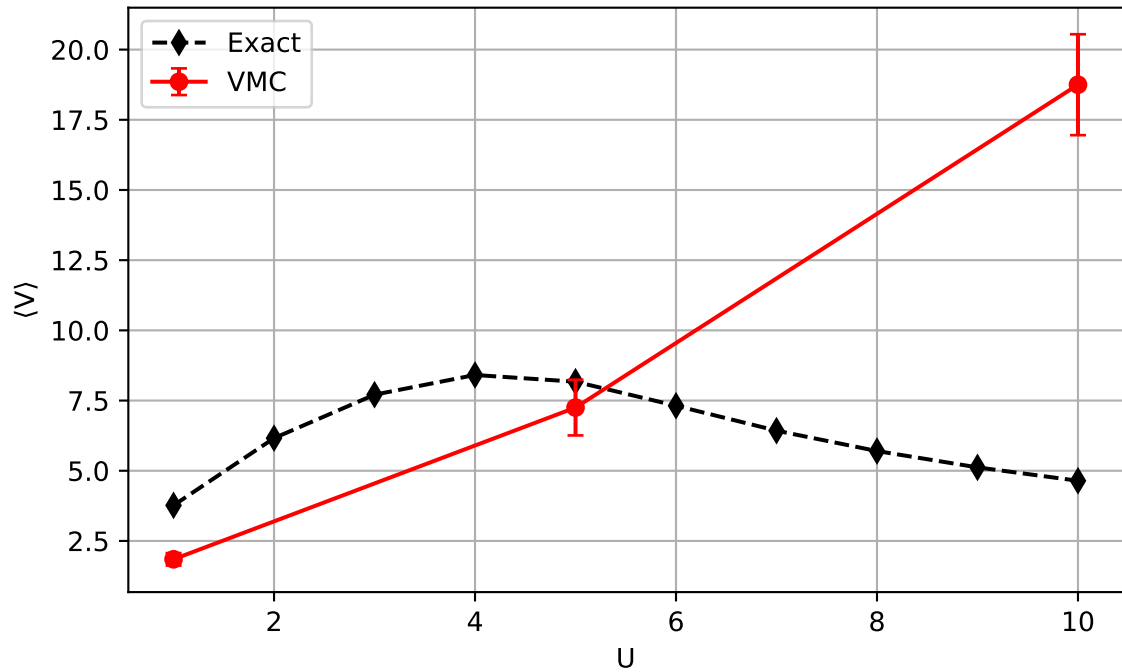
1D, L12, N12 - Potential Energy
