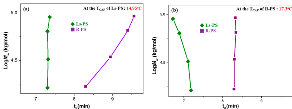
Figure 9. Log MW vs elution time plot of Ls-PS and Ring-PS at (a) T_{\text{CAP}}(\text{Ls-PS}) and at (b) T_{\text{CAP}}(\text{Ring-PS}) .
