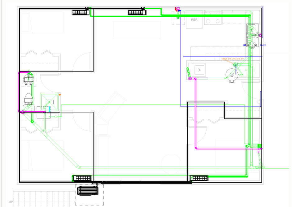
ENCL. 05-C · SANITARY DRAINAGE AND VENT
