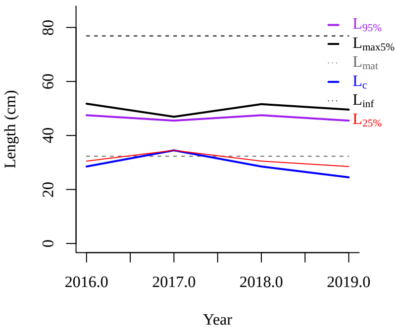
(c) Optimal Yield
