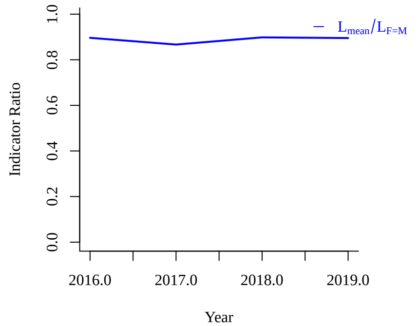
(f) Maximum sustainable yield
