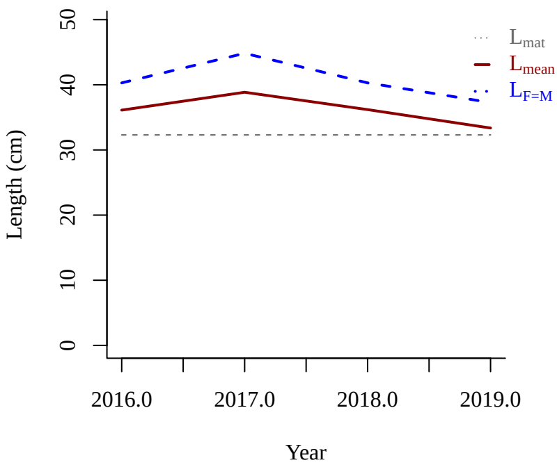
(e) Maximum Sustainable Yield
