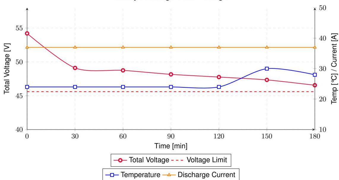
Battery Discharge Curve - String 1
