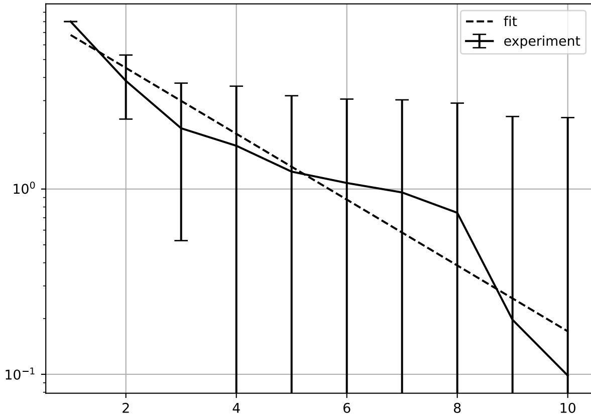
1-particle Heisenberg model on 56 qubits
