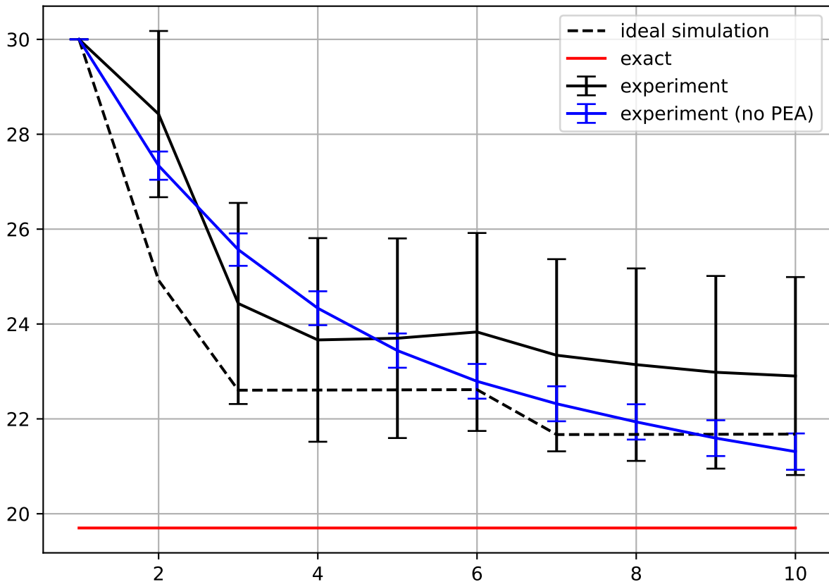
3-particle Heisenberg model on 44 qubits
