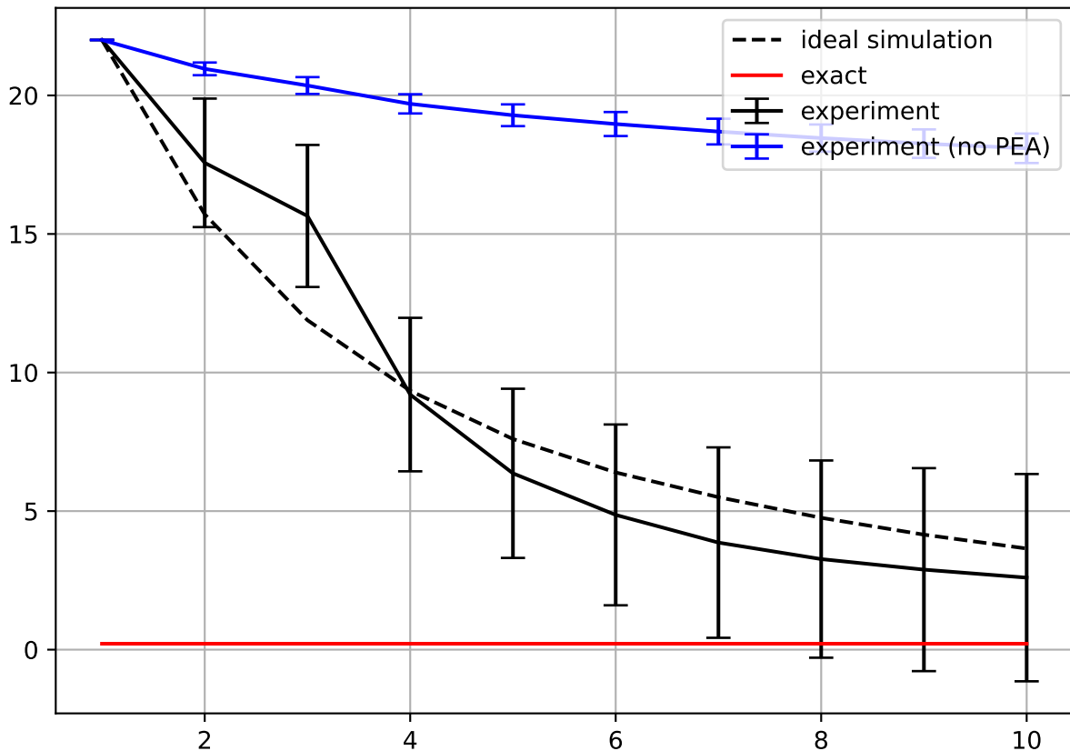
5-particle Heisenberg model on 42 qubits
