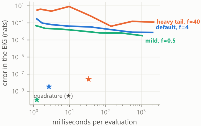
(a) what accuracy costs
