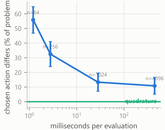
(c) whether it reaches the decision
