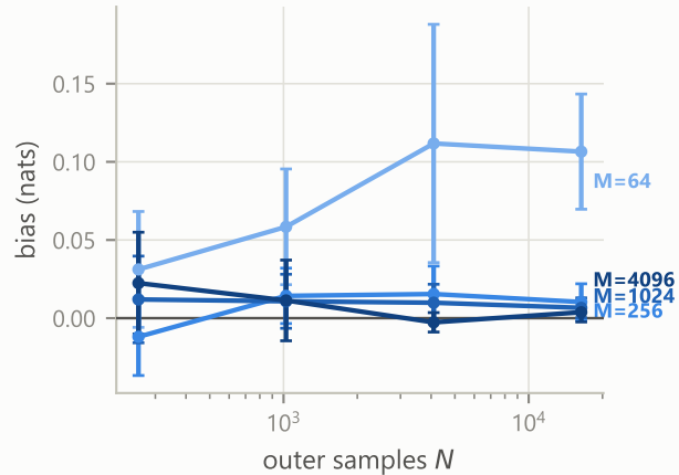
(b) the bias is set by M , not N
