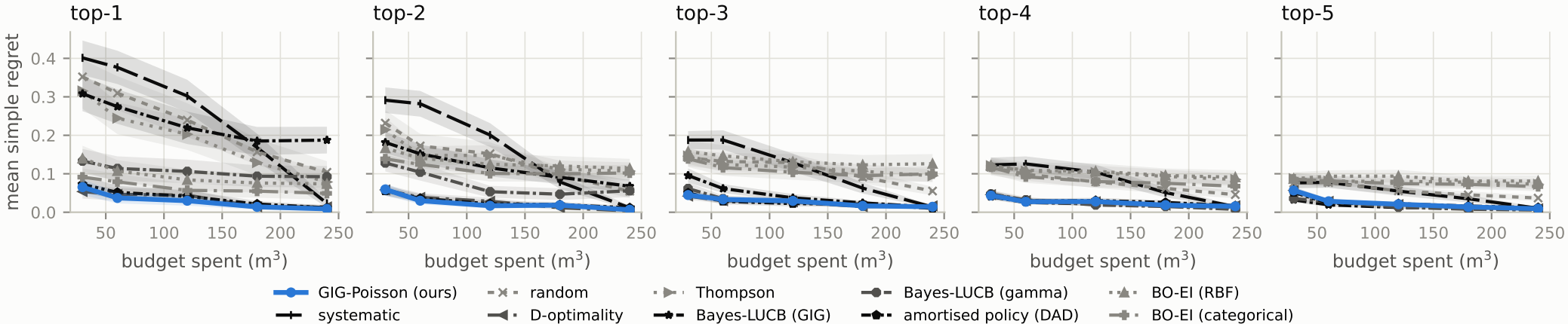
Bulk sampling (acquisitions): top-m regret (shaded: \pm 1 s.e. over 50 runs)
