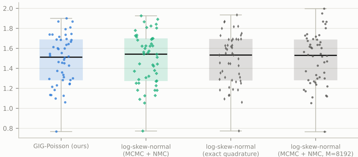
Bulk sampling (appendix_Isn): held-out NLPD at the full budget (240 m 3 ), 50 runs
