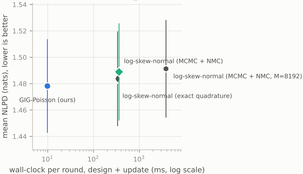
Bulk sampling (appendix_Isn): accuracy against cost, 50 runs
