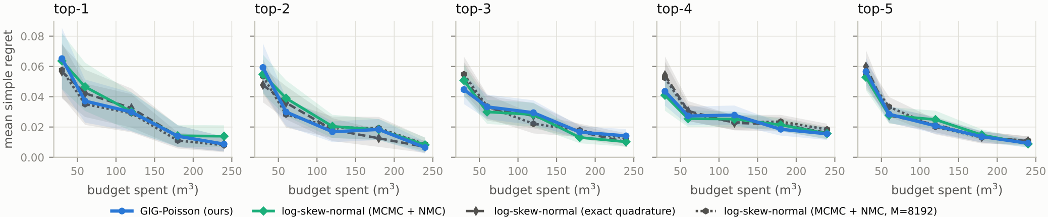
Bulk sampling (appendix_1sn): top-m regret (shaded: \pm 1 s.e. over 50 runs)
