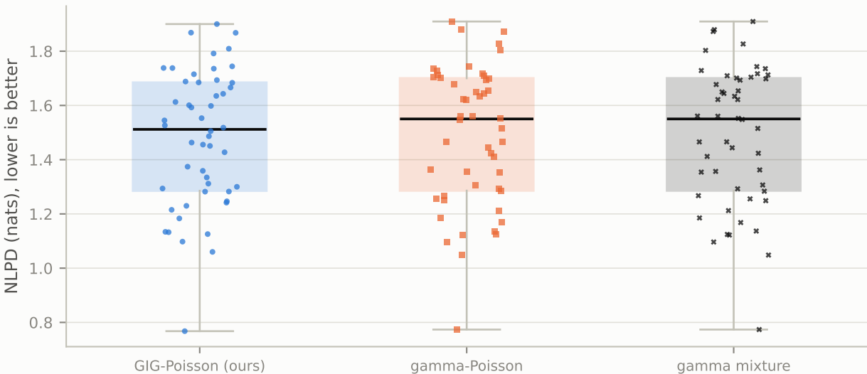
Bulk sampling (models): held-out NLPD at the full budget (240 m 3 ), 50 runs
