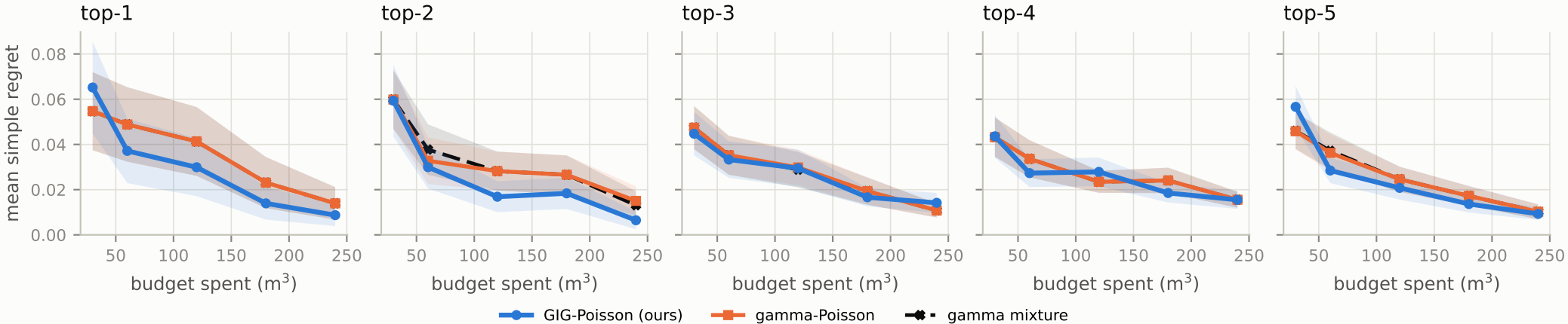
Bulk sampling (models): top-m regret (shaded: \pm 1 s.e. over 50 runs)
