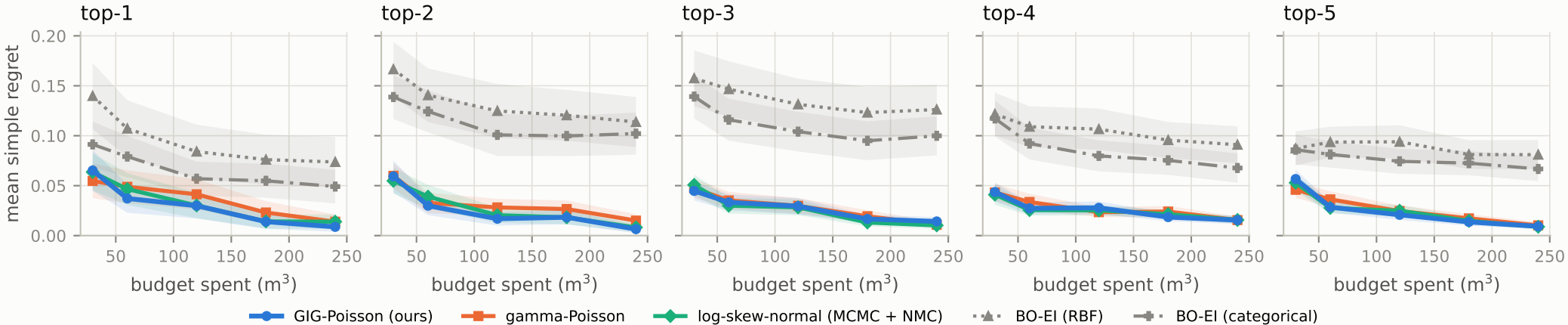
Bulk sampling: top-m regret (shaded: \pm 1 s.e. over 50 runs)
