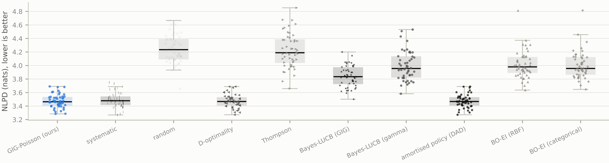
Gamma-ray, 1-99% flux band (acquisitions): held-out NLPD at the full budget (120 Ms), 50 runs
