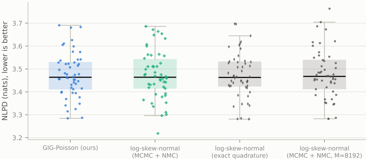
Gamma-ray, 1-99% flux band (appendix_lsn): held-out NLPD at the full budget (120 Ms), 50 runs
