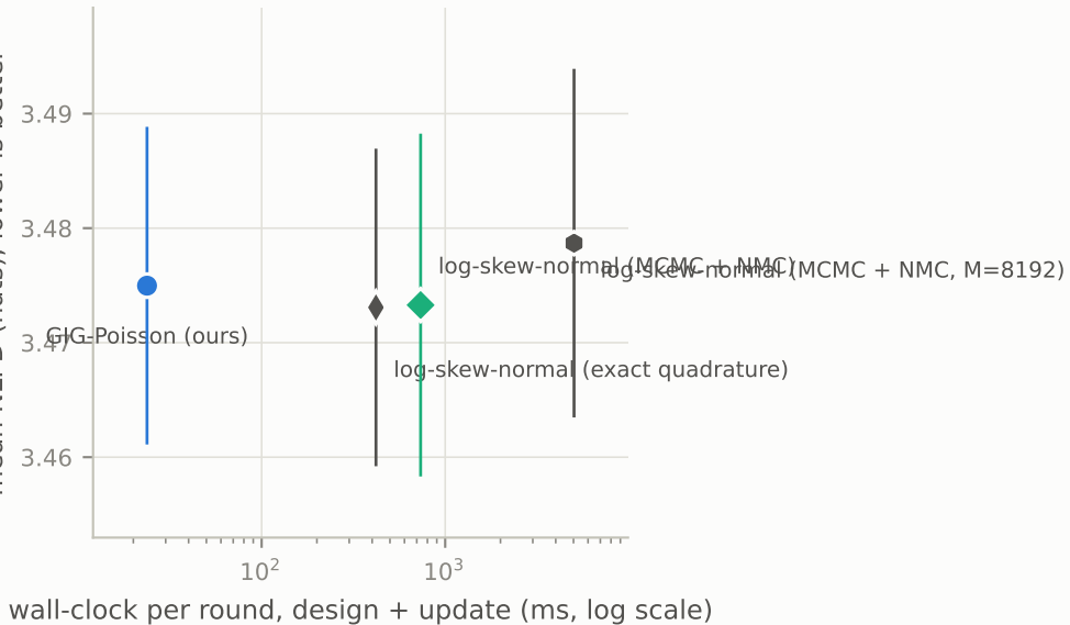
Gamma-ray, 1-99% flux band (appendix_lsn): accuracy against cost, 50 runs
