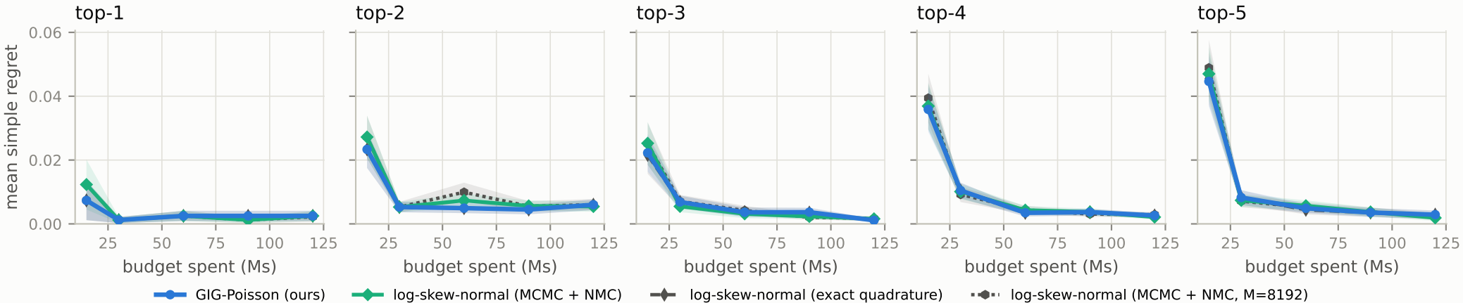
Gamma-ray, 1-99% flux band (appendix_Isn): top-m regret (shaded: \pm 1 s.e. over 50 runs)
