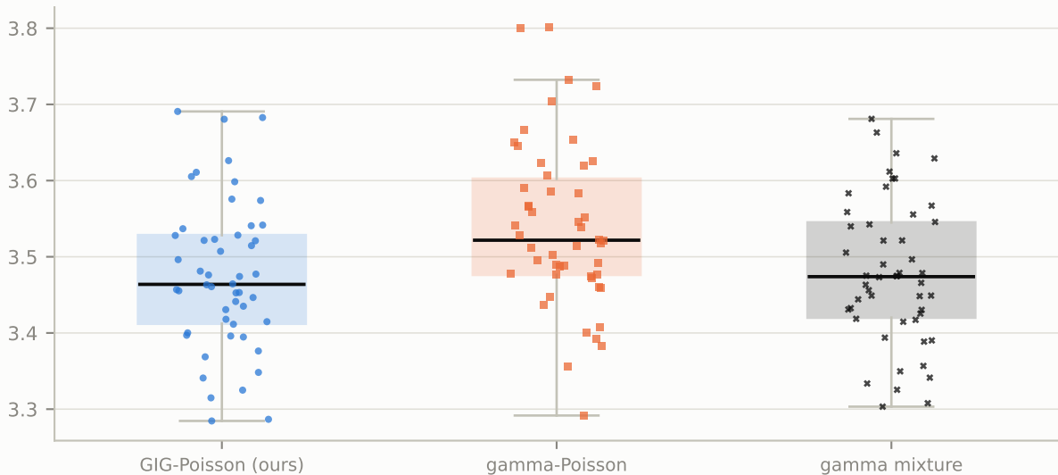
Gamma-ray, 1-99% flux band (models): held-out NLPD at the full budget (120 Ms), 50 runs
