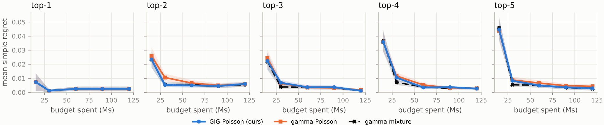
Gamma-ray, 1-99% flux band (models): top-m regret (shaded: \pm 1 s.e. over 50 runs)
