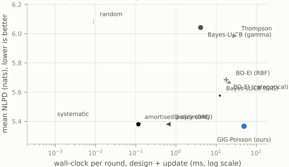
Gamma-ray survey: 192 targets, scored at 25 Ms (acquisitions): accuracy against cost, 50 runs
