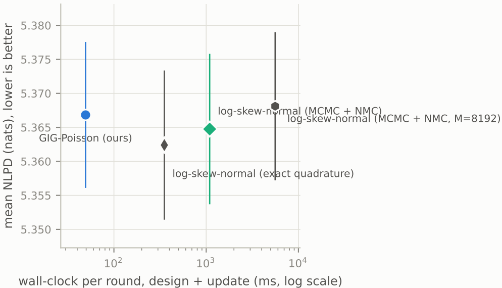
Gamma-ray survey: 192 targets, scored at 25 Ms (appendix_1sn): accuracy against cost, 50 runs
