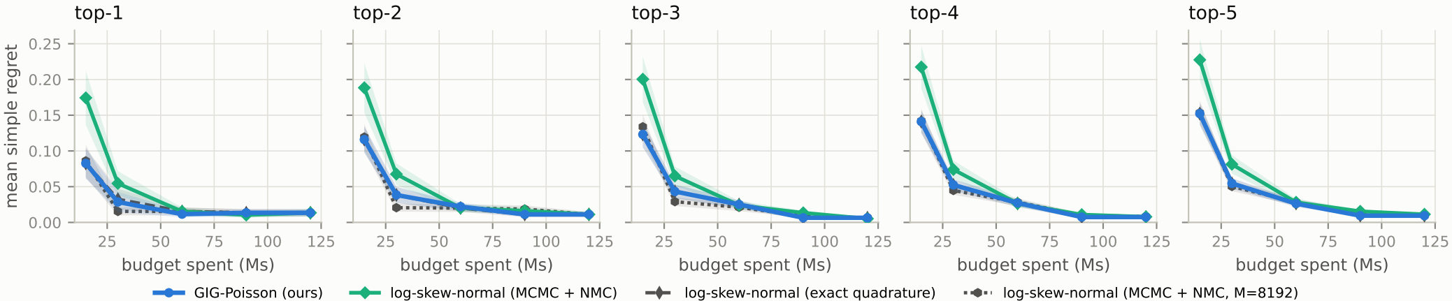
Gamma-ray survey: 192 targets, scored at 25 Ms (appendix_Isn): top-m regret (shaded: \pm 1 s.e. over 50 runs)
