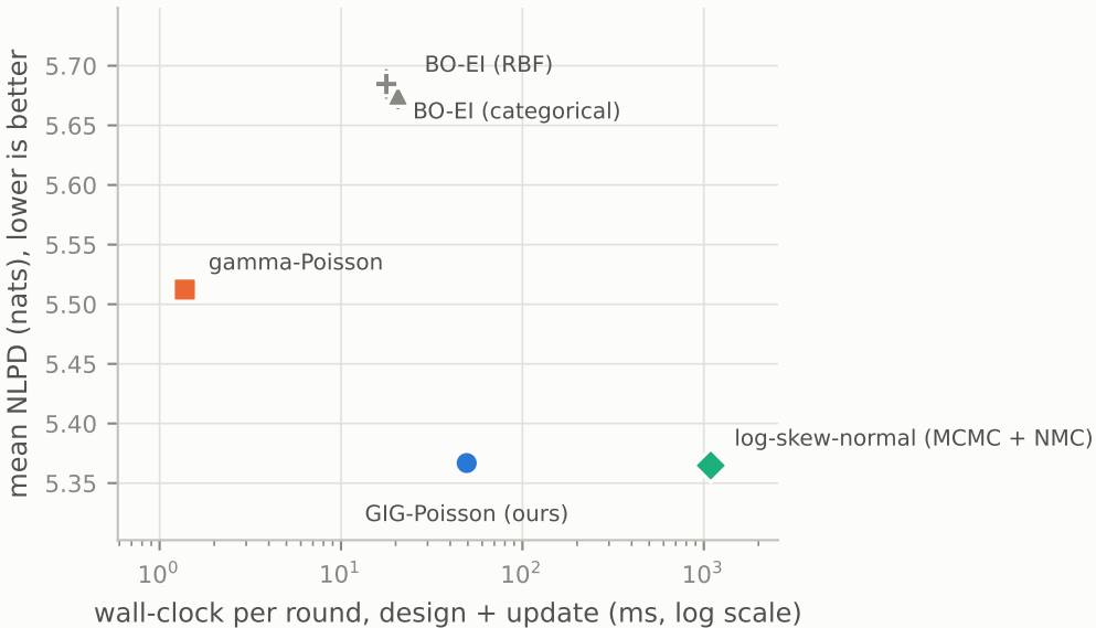
Gamma-ray survey: 192 targets, scored at 25 Ms: accuracy against cost, 50 runs
