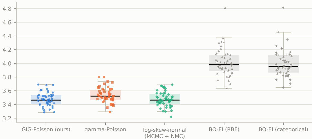
Gamma-ray, 1-99% flux band: held-out NLPD at the full budget (120 Ms), 50 runs
