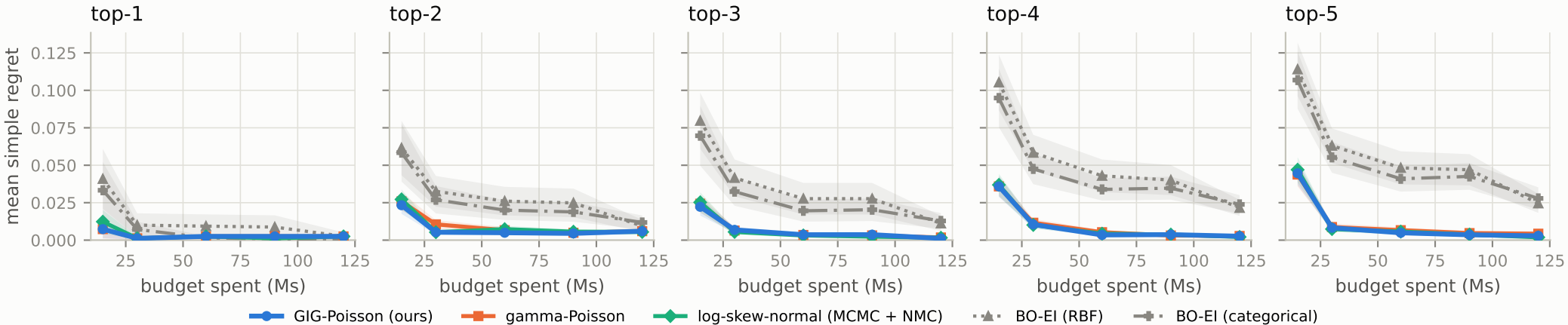
Gamma-ray, 1-99% flux band: top-m regret (shaded: \pm 1 s.e. over 50 runs)
