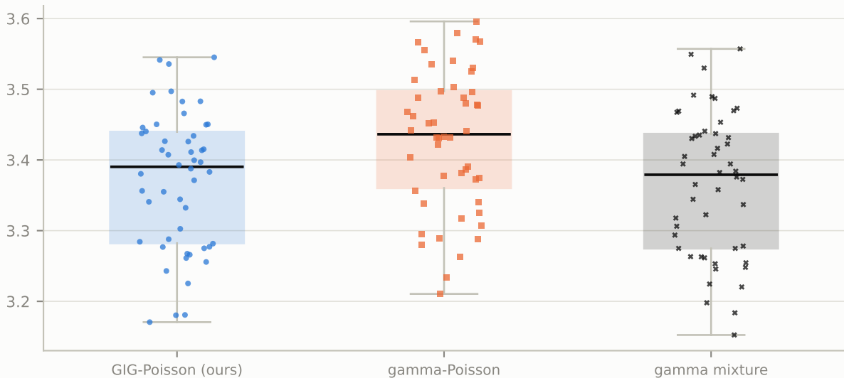
Gamma-ray, 5-95% flux band (models): held-out NLPD at the full budget (120 Ms), 50 runs
