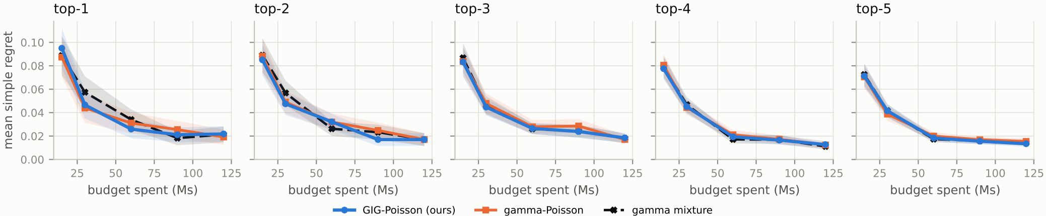
Gamma-ray, 5-95% flux band (models): top-m regret (shaded: \pm 1 s.e. over 50 runs)
