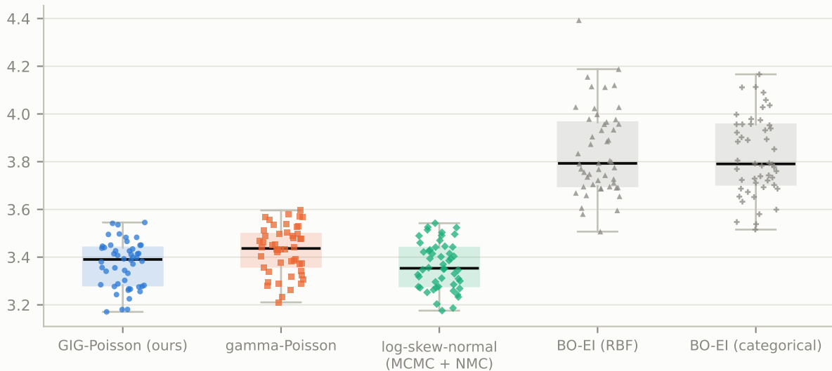
Gamma-ray, 5-95% flux band: held-out NLPD at the full budget (120 Ms), 50 runs
