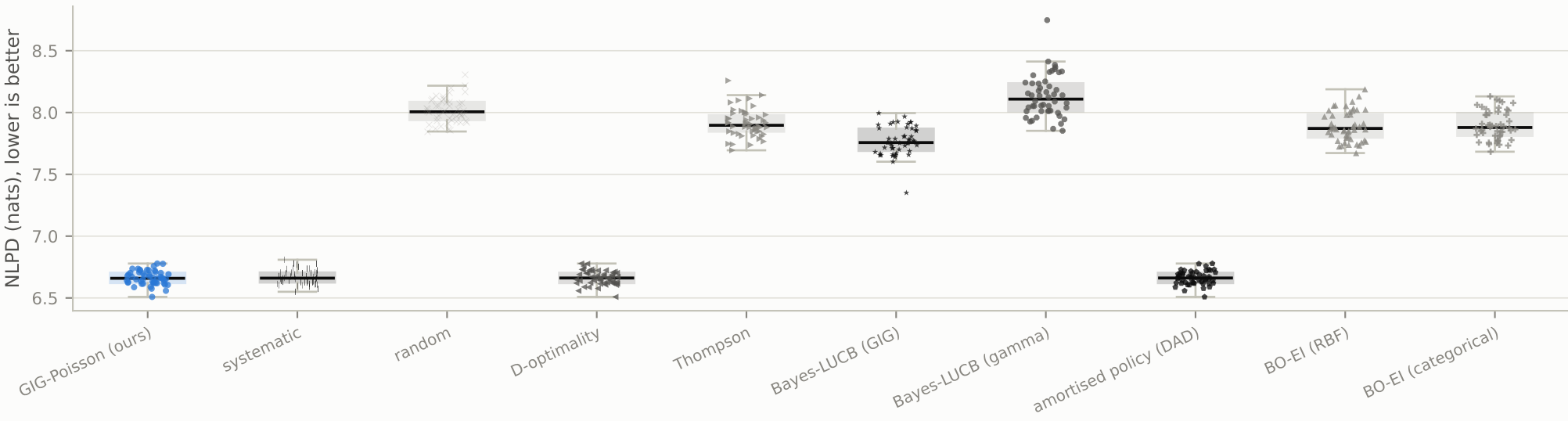
Hard X-ray follow-up of Swift-BAT sources (acquisitions): held-out NLPD at the full budget (120 ks), 50 runs
