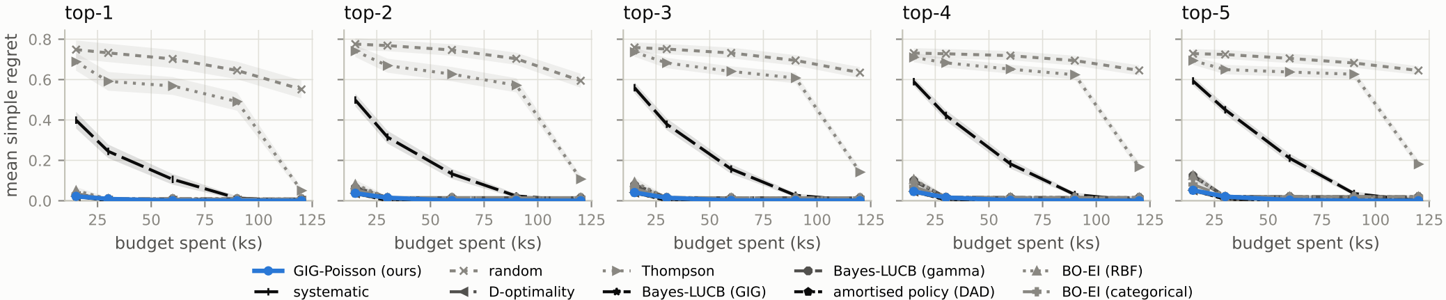
Hard X-ray follow-up of Swift-BAT sources (acquisitions): top-m regret (shaded: \pm 1 s.e. over 50 runs)
