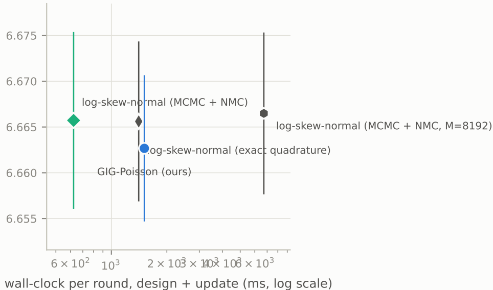
Hard X-ray follow-up of Swift-BAT sources (appendix_Isn): accuracy against cost, 50 runs
