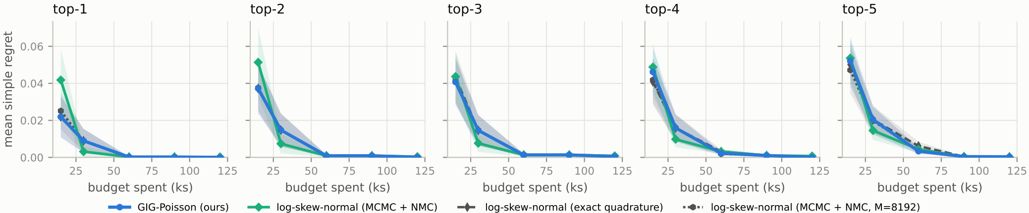
Hard X-ray follow-up of Swift-BAT sources (appendix_Isn): top-m regret (shaded: \pm 1 s.e. over 50 runs)
