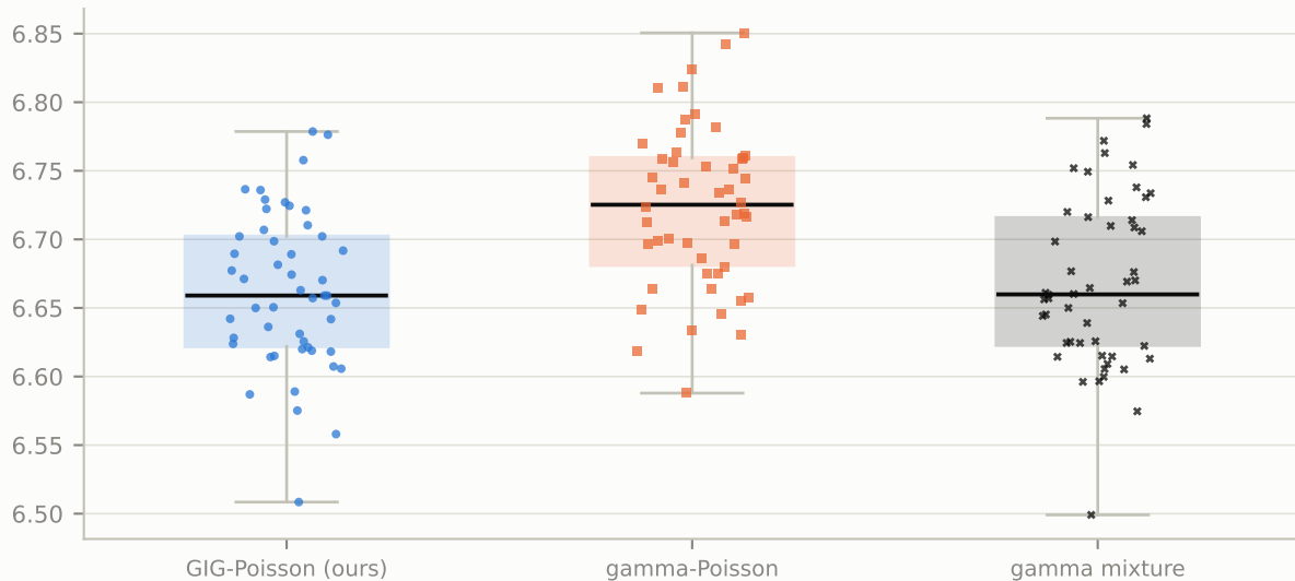
Hard X-ray follow-up of Swift-BAT sources (models): held-out NLPD at the full budget (120 ks), 50 runs
