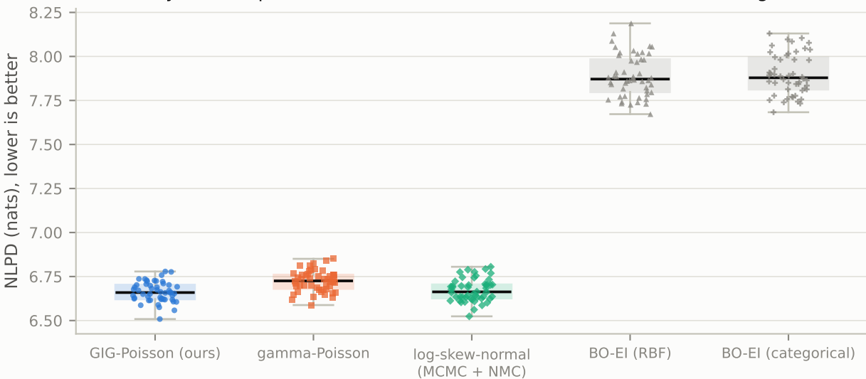
Hard X-ray follow-up of Swift-BAT sources: held-out NLPD at the full budget (120 ks), 50 runs
