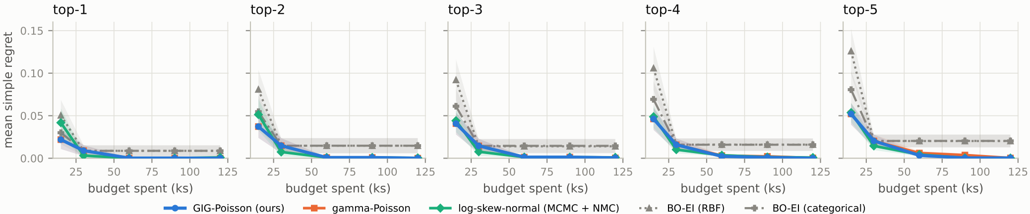
Hard X-ray follow-up of Swift-BAT sources: top-m regret (shaded: \pm 1 s.e. over 50 runs)
