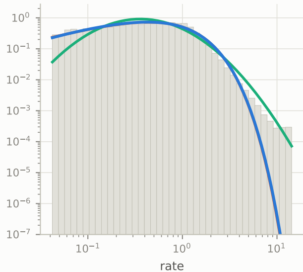
20 Newsgroups terms n = 22460 , fitted order +1.73
