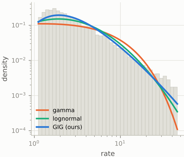
Fermi-LAT sources n = 4557 , fitted order -1.43
