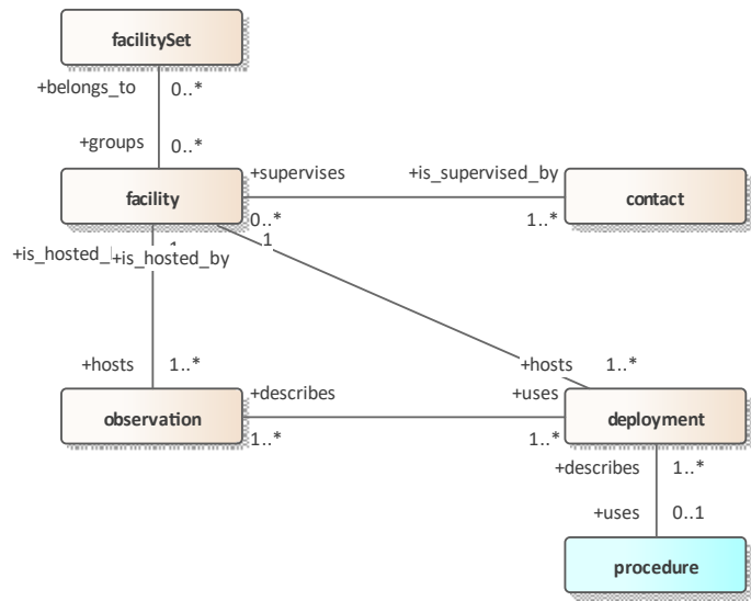
Figure 2: WMDR2-core-logical
