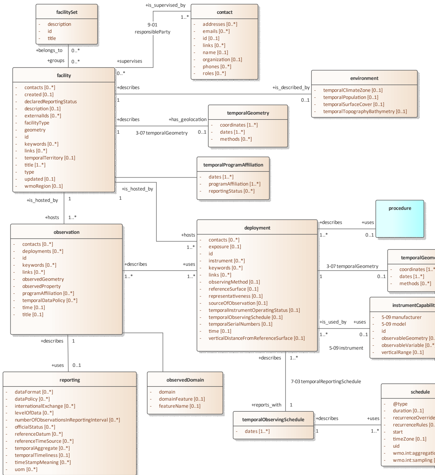
Figure 1: WMDR2-core
