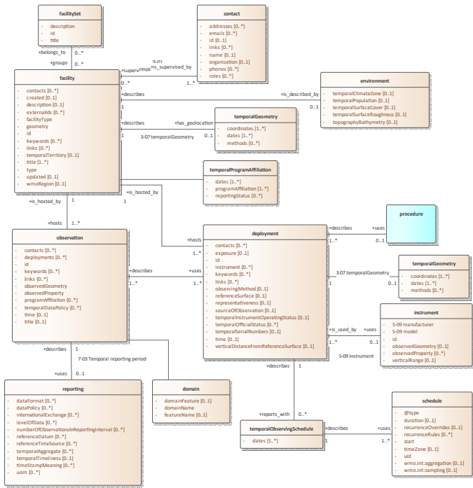
Figure 1: WMDR2-core
